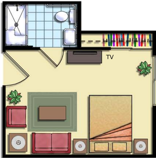
PRIVATE SUITE 290 s.f. (17'-6" x 16'-0")
